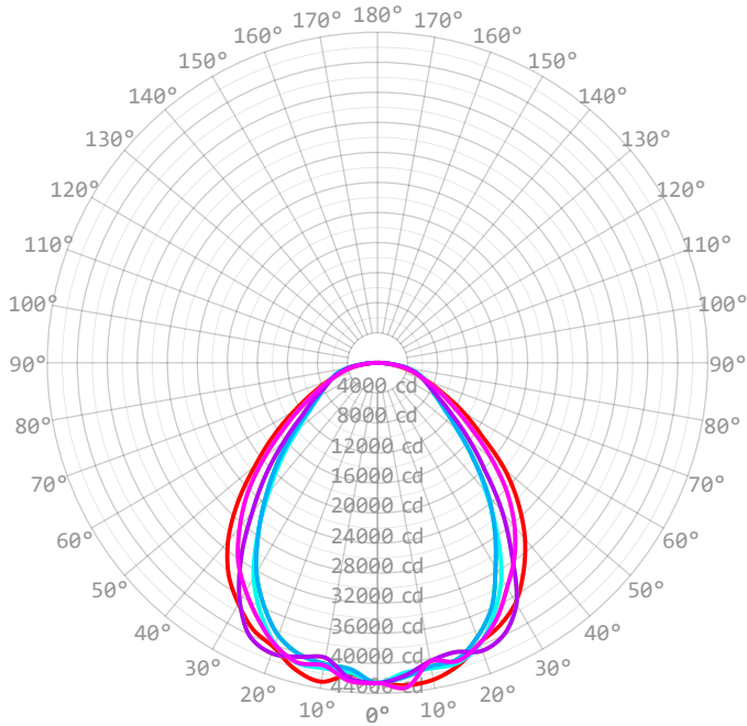
Based on 'BLHJ-4FT-96L-850-L82' ie. (BLHJ, 4 foot, 96000lm, 80 CRI, 5000K, w/ L82 10x60 Aisle Lens)
