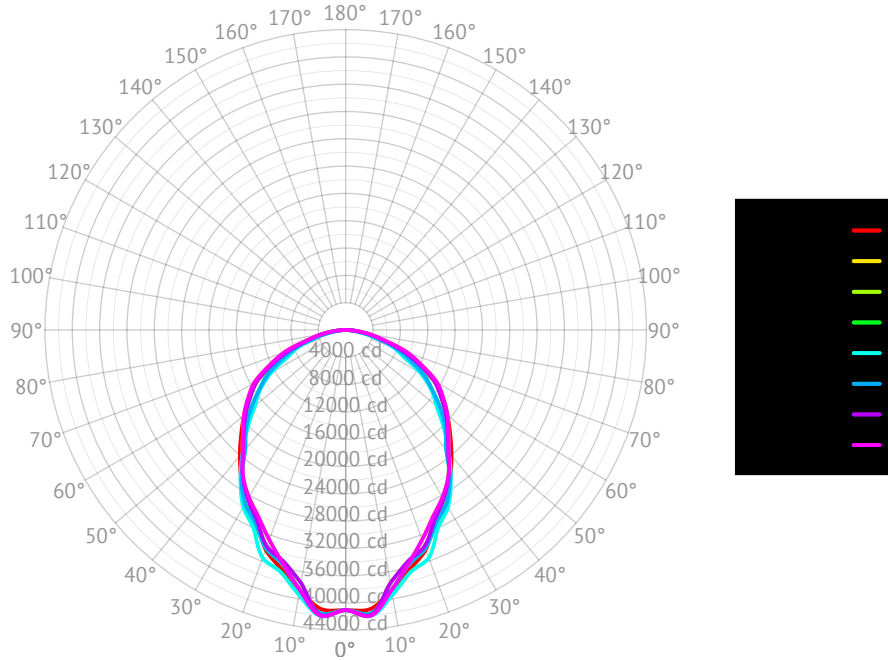
Based on 'BLHJ-4FT-96L-850-L69' ie. (BLHJ, 4 foot, 96000lm, 80 CRI, 5000K, w/ L69 Lens)
